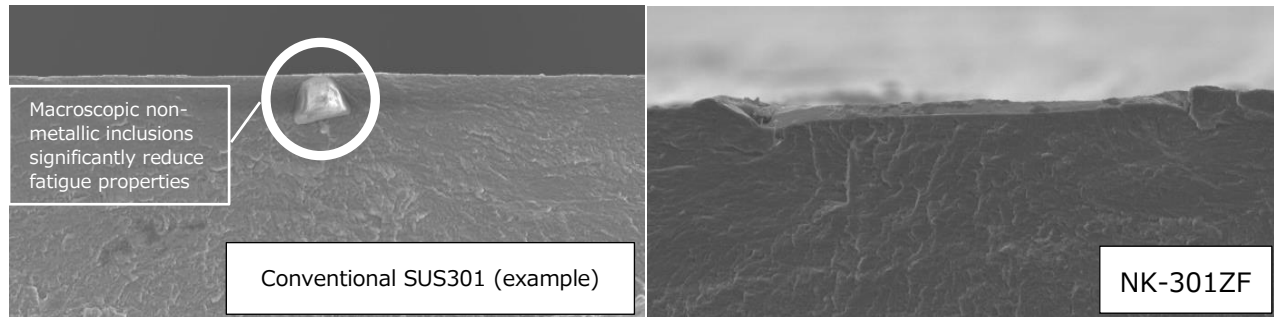
Fig.3 Image of Inclusions
