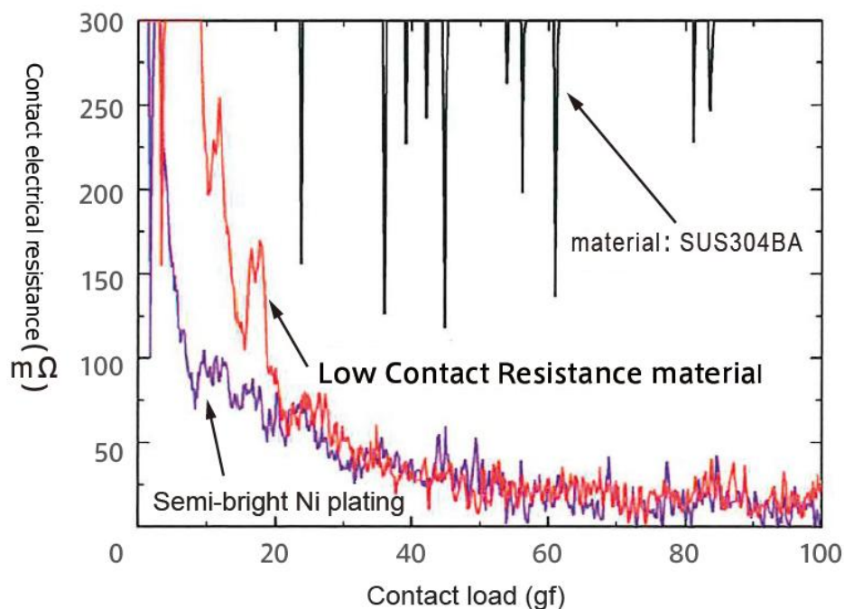
Figure 2: Comparison between Base Material (SUS304 BA) and Semi-bright Ni-plated Material
